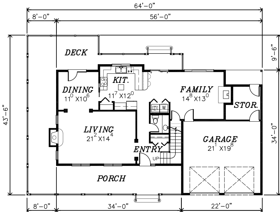
MAIN FLOOR PLAN 1,086 SQ.FT.
