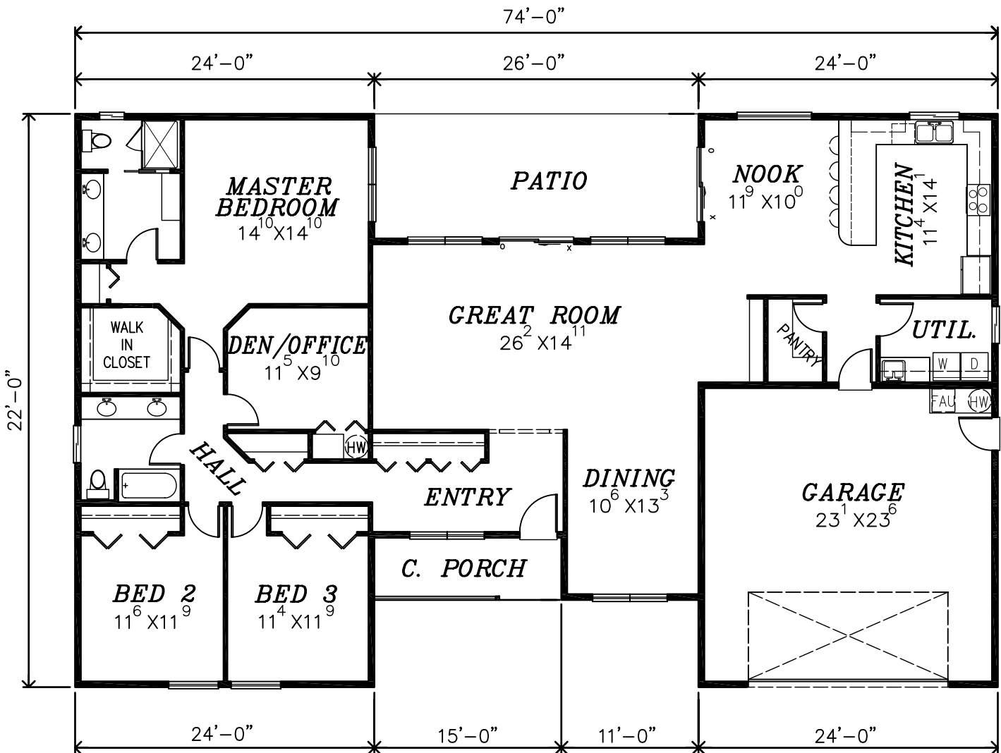
MAIN FLOOR PLAN 2,319 SQ.FT.
