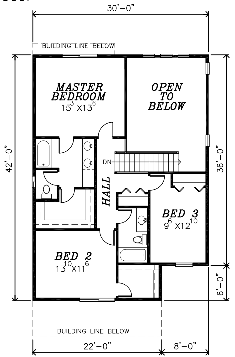
UPPER FLOOR PLAN 926 SQ.FT.
