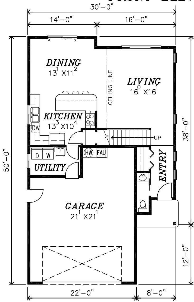
MAIN FLOOR PLAN 808 SQ.FT.
