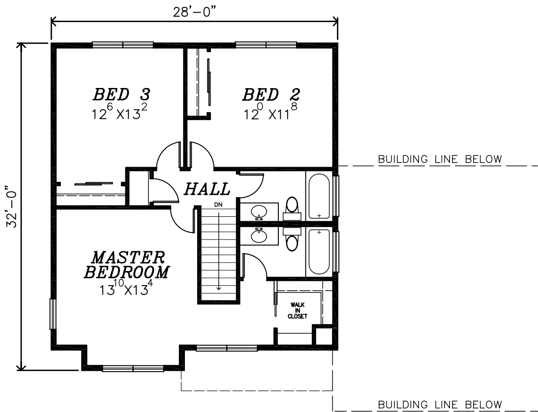
UPPER FLOOR PLAN 826 SQ.FT.
