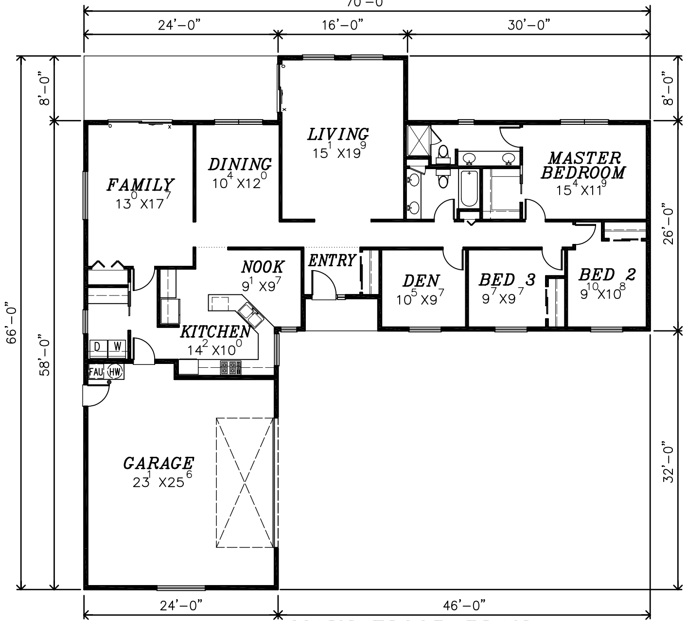
MAIN FLOOR PLAN 2,034 SQ.FT.
