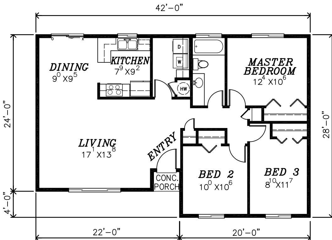
MAIN FLOOR PLAN 1,076 SQ.FT.
