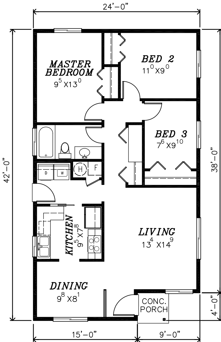
MAIN FLOOR PLAN 972 SQ.FT.
