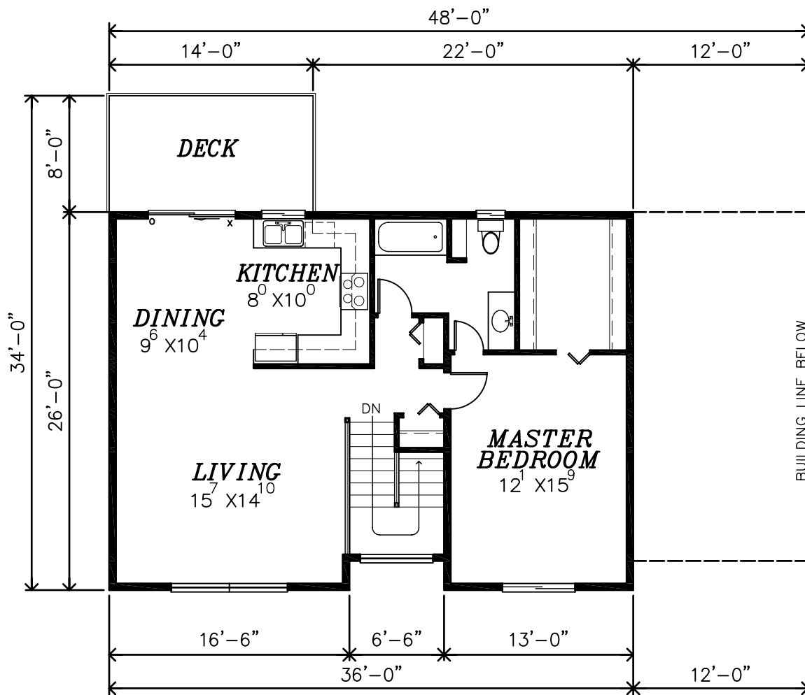
UPPER FLOOR PLAN 923 SQ.FT.
