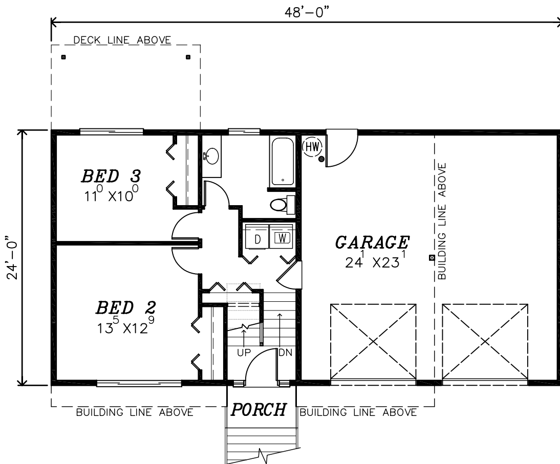
LOWER FLOOR PLAN 504 SQ.FT.
